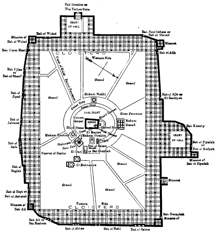
PLAN OF KAABA
